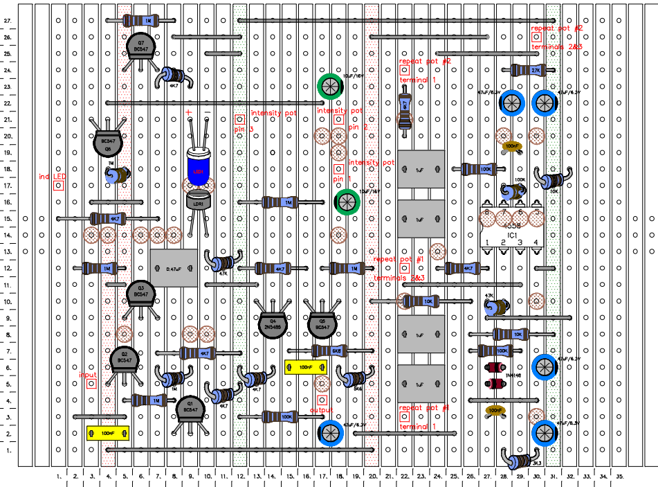
top component side
